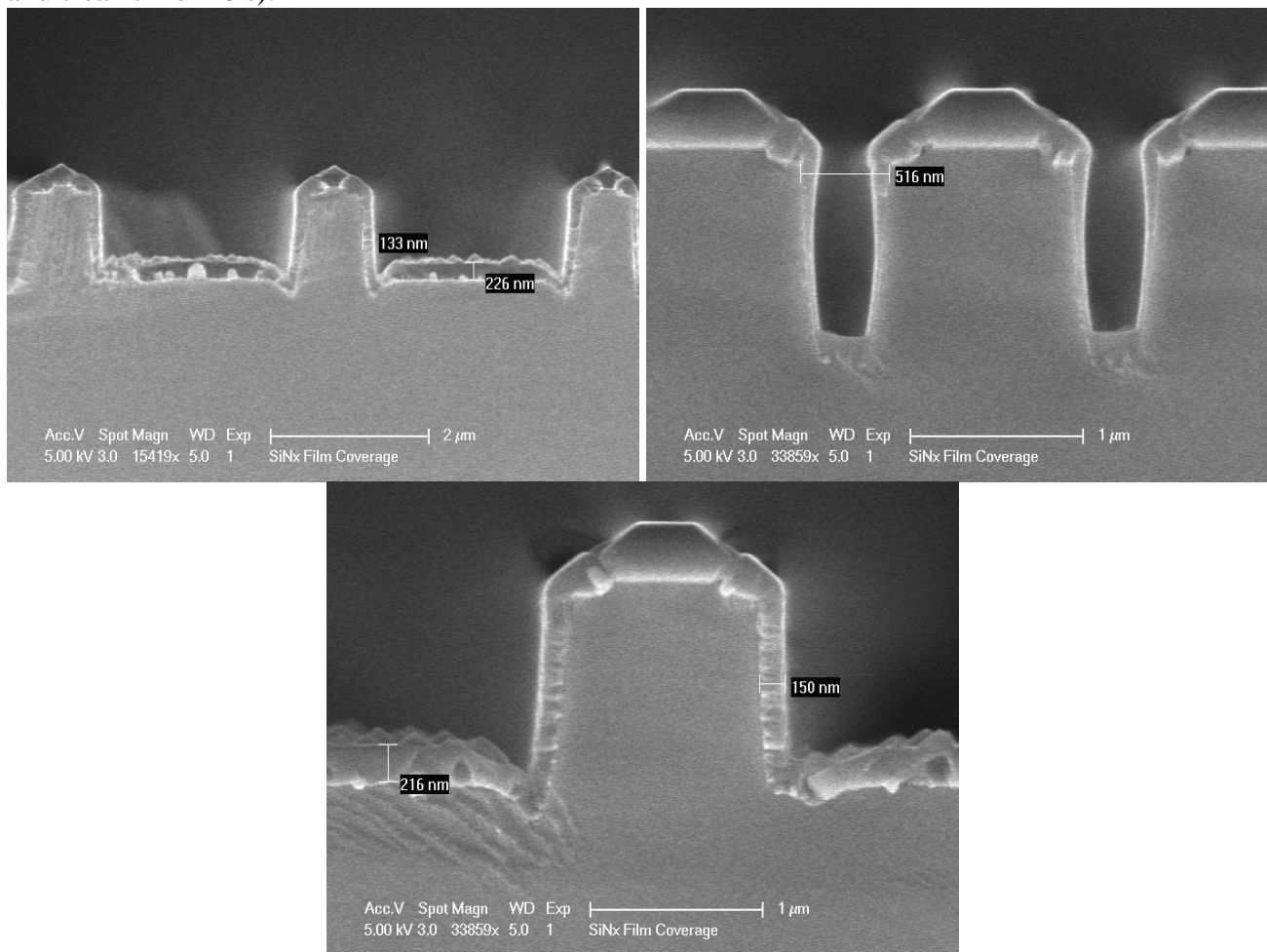
Figure (a), (b), and (c) Side wall coverage of medium-stress SiNx film, deposited using Unaxis ICP tool at 100 °C, with chamber pressure=10 mT, bias/ICP powers=50 (94 V)/800 W, 100% SiH 4 /N 2 /Ar=15.5/8.5/20 sccm, and deposition time=266 s (One-minute buffered HF dip and Ar plasma clean prior to the deposition with pressure=10 mT, Ar flow rate=30 sccm, bias/ICP powers=20/800 W, and clean time=40 s).
